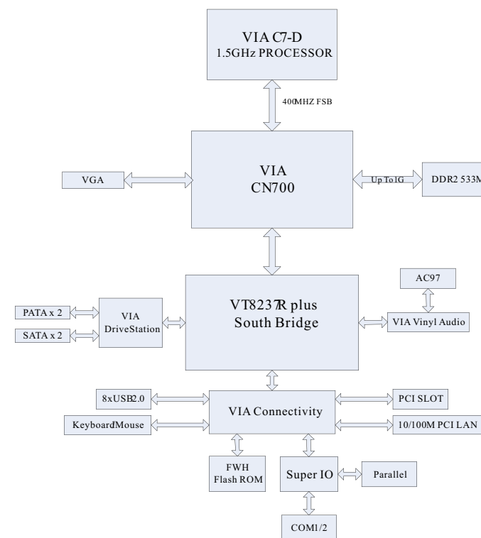
EC7-8721CNA FUNCTION BLOCK DIAGRAM
