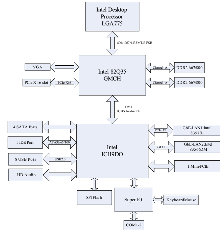
EC7-8815V2NA FUNCTION BLOCK DIAGRAM
