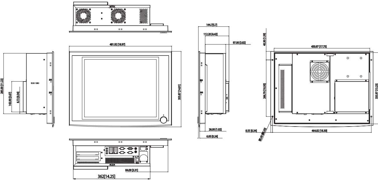
Panel Cut-out Dimensions: 454 x 338 mm
